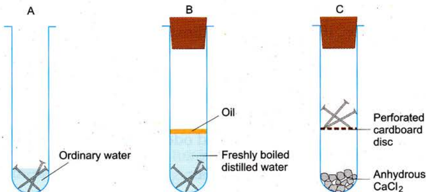
Fig. 4.3 Only moist air causes rusting.
