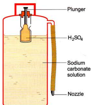
Fig. 4.12 A fire extinguisher
