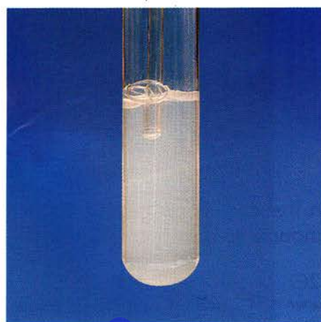
Fig. 4.11 Carbon dioxide turns limewater milky.
